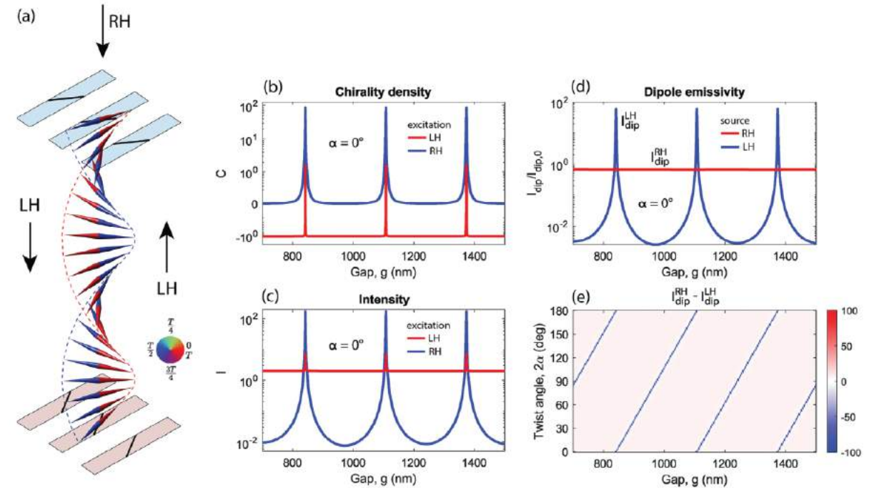
Figure 3. a) Sketch view of a chiral resonator supporting LH Fabry–Pérot modes. The cones represent electric vectors of the incident wave settled in the gap between the mirrors, with phases specified by the circular colorbar. The field distribution is calculated for the gap size g \approx 575 nm and the twist angle 2\alpha = 0^\circ . The gap-size dependence of b) the time-average normalized chirality density and c) normalized intensity in the middle of the cavity. d) The gap-size dependence of the emissivity of RH and LH dipole sources placed in the middle of the cavity. e) The gap-size and twist-angle dependence of a difference between RH and LH dipole emissivities.
